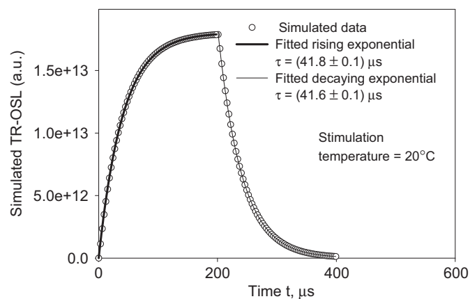
Fig. 2. Simulated time resolved spectrum for quartz using the model shown in Fig. 1. The LED stimulation is ON for 200 \text{ } \mu\text{s} and OFF for the same amount of time. The rising and decaying parts of the signal are fitted with a rising exponential and a decaying exponential correspondingly.
