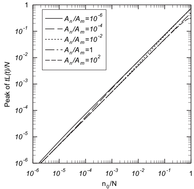
Fig. 1. The peak of the normalized transformed LM-OSL, tL/N , plotted against the normalized initial concentration, n_0/N for various values of \hat{A} = A_n/A_m . The slight changes in the y-axis for the other luminescence expressions are explained in the text.
