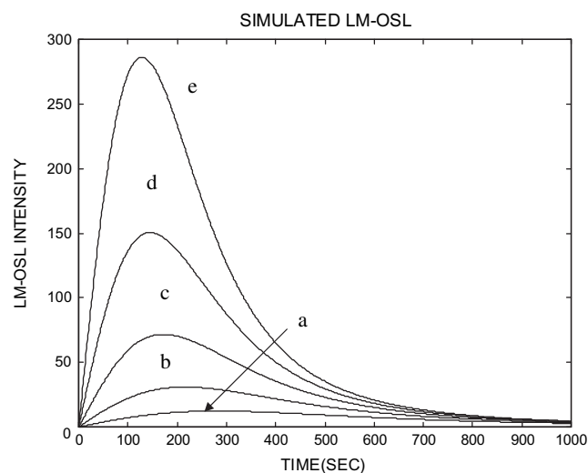
Fig. 4. Simulated LM-OSL curves for the same set of parameters as in Fig. 3. Excitation times are 1, 2, 4, 8, 16 s in curves a, b, c, d and e, respectively.
