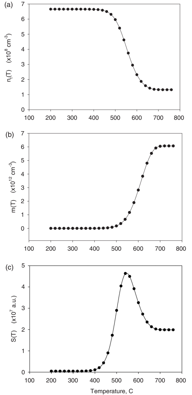
Figure 4. For a chosen set of parameters, n_t at the end of the test-dose excitation as a function of the activation temperature T is shown on (a); the occupancy of the recombination centres as a function of T is shown in (b) and the resulting sensitivity S(T) is given in (c). The parameters are given in the text.
